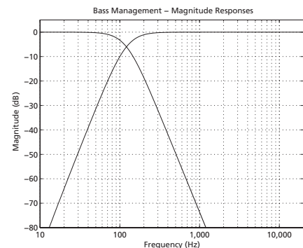
Figure 8: Magnitude response of the crossover used in the Bass Management system, showing an example with default frequency of 120 Hz.
