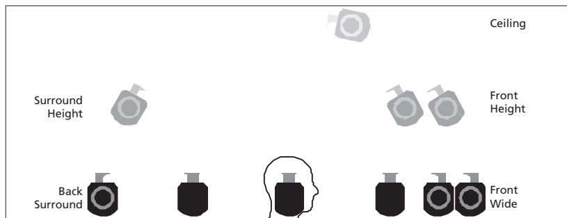
Figure 6: Side view of the loudspeaker positions associated with the speaker roles available in the television
