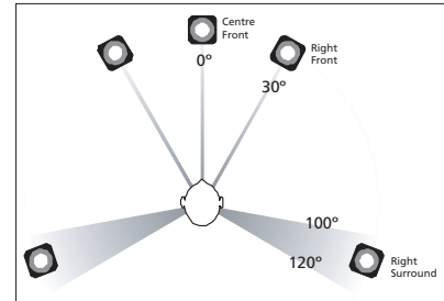
Figure 12: Standard loudspeaker configuration for 5.1 multichannel audio. The actual placement of the surround loudspeakers (at 110 deg) shows the reference placement used at Bang & Olufsen for testing and tuning. Note that the placement of the subwoofer is better determined by your listening room's acoustics, but it is advisable to begin with a location near the centre front loudspeaker, if possible.
