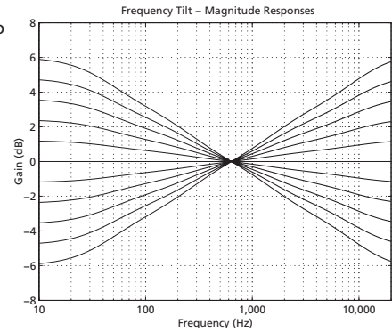
Figure 1: Frequency response measurements of all settings of the Frequency Tilt control. Note that this response is applied to each input channel.
