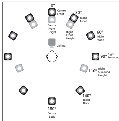
Figure 5: Loudspeaker positions associated with the speaker roles available in the television. The Truelmage processor delivers a unique output to each of these output channels.
