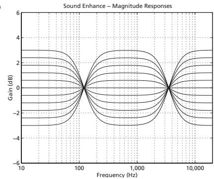
Figure 2: Frequency response measurements of all settings of the Sound Enhance control. Note that this response is applied to each input channel.
