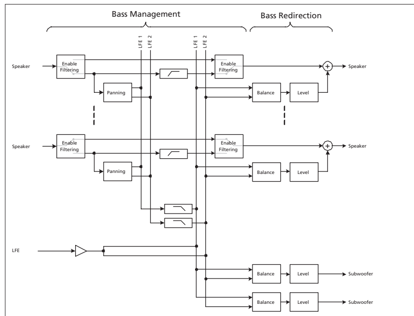
Figure 7: Block diagram of the Bass Management and Bass Re-direction processing in the television.
